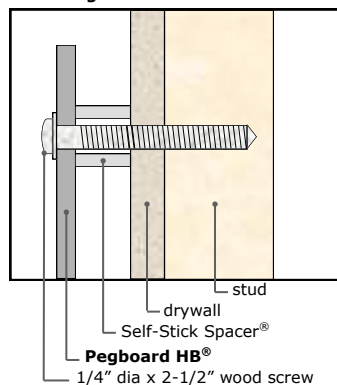
Fastening into wall stud
