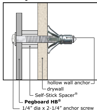
Fastening into hollow wall
