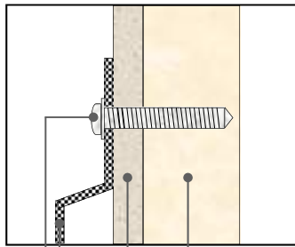
drywall stud PegBoard Strip™ 1/4" dia x 2-1/2" wood screw
